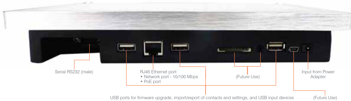
Touch Panel Controller Bottom panel
