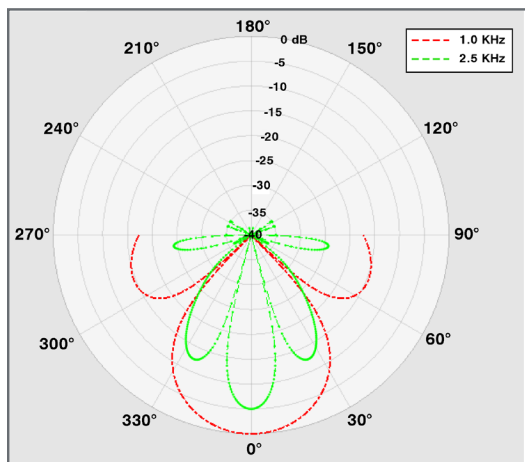
Typical Beamforming
