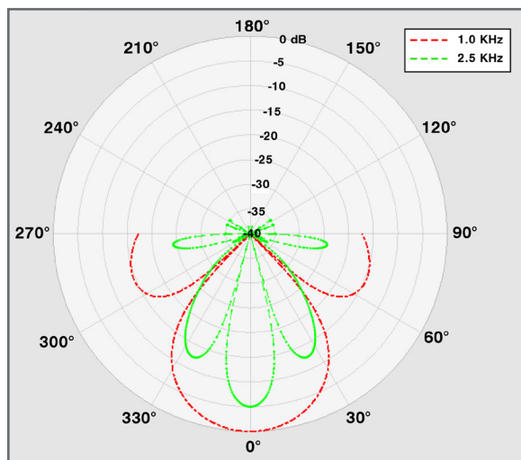
Typical Beamforming
