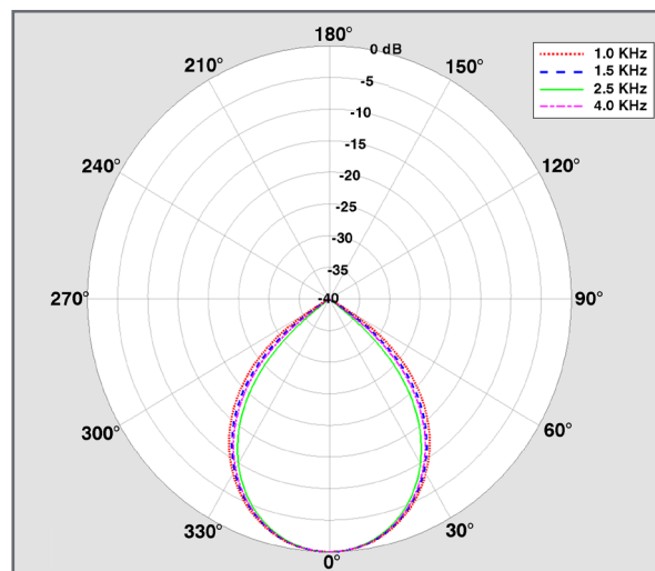
ClearOne BMA 360 Beamforming with FiBeam and DsBeam
