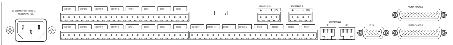
XAP 800 Rear Panel
