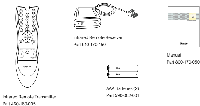
Figure 1. XAP IR Remote Control System
