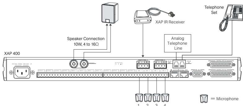
Figure 4. Typical XAP IR Remote Receiver installation
