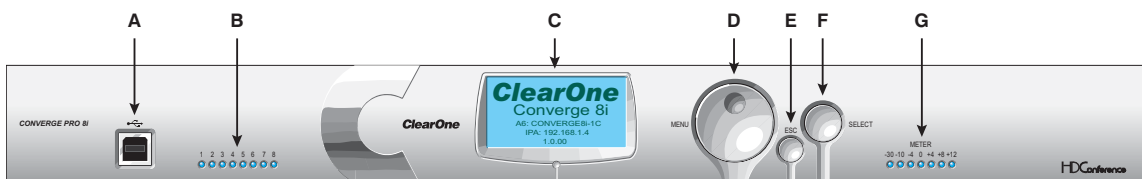
Converge Pro 8i Front Panel
