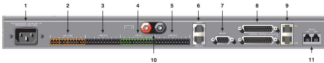
Converge Pro 840T Rear Panel
