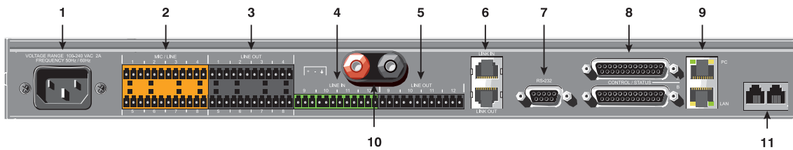
Converge Pro 840T Rear Panel
