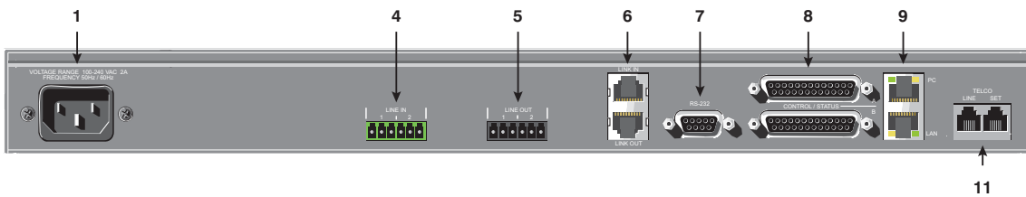
Converge Pro TH20 Rear Panel
